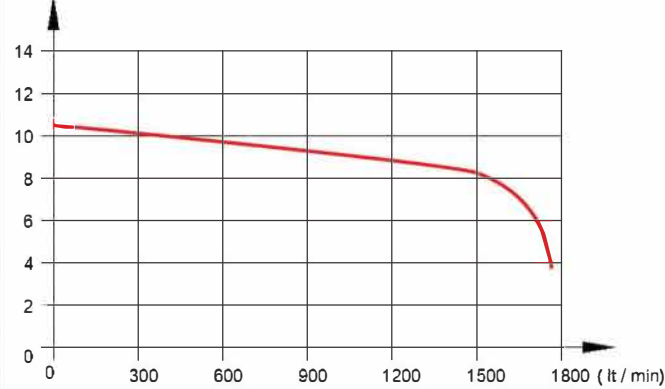
Pressure (Bar) Diagram of Pump Performance
