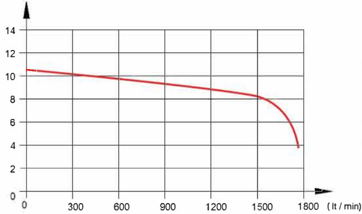
Pressure (Bar) Diagram of Pump Performance
